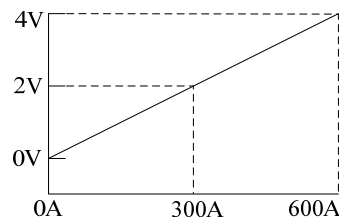
输出曲线对应图 Output Curve Diagram
