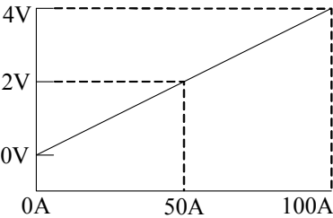
输出曲线对应图 Output Curve Diagram
