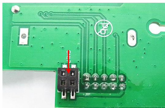
4.4 (客户参考图片 (非测试样品)) (Client Reference Photo(Non-tested sample))
