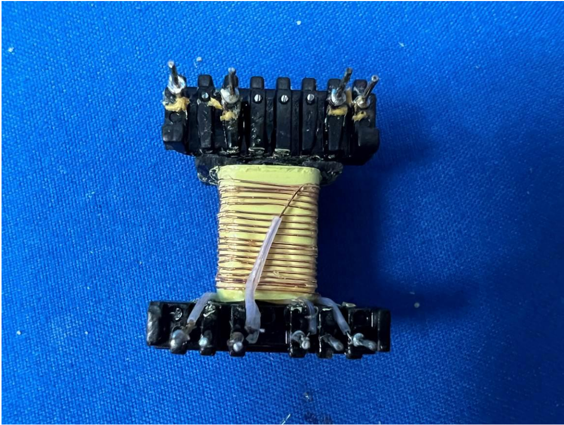
Primary winding
