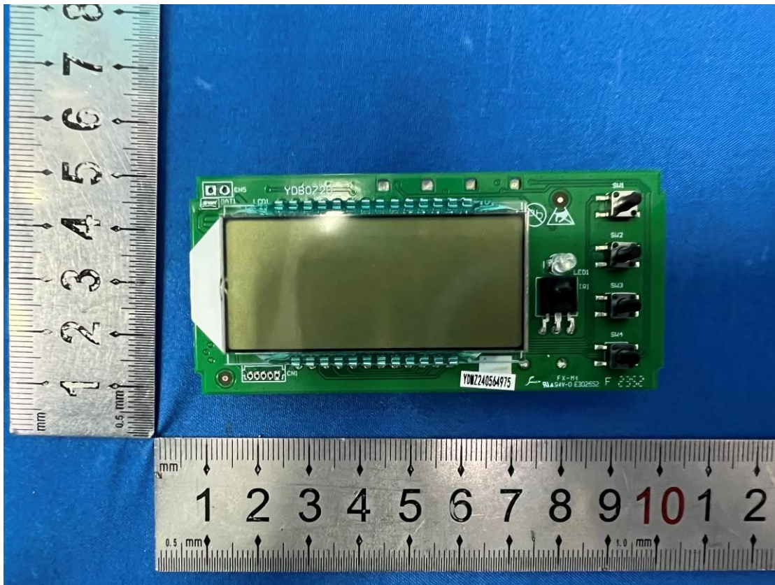
YDB072D board view
