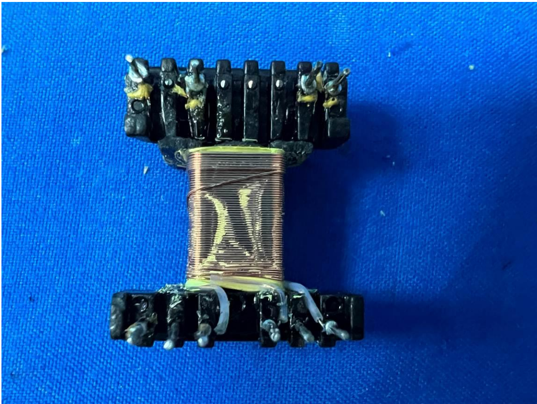
Primary winding
