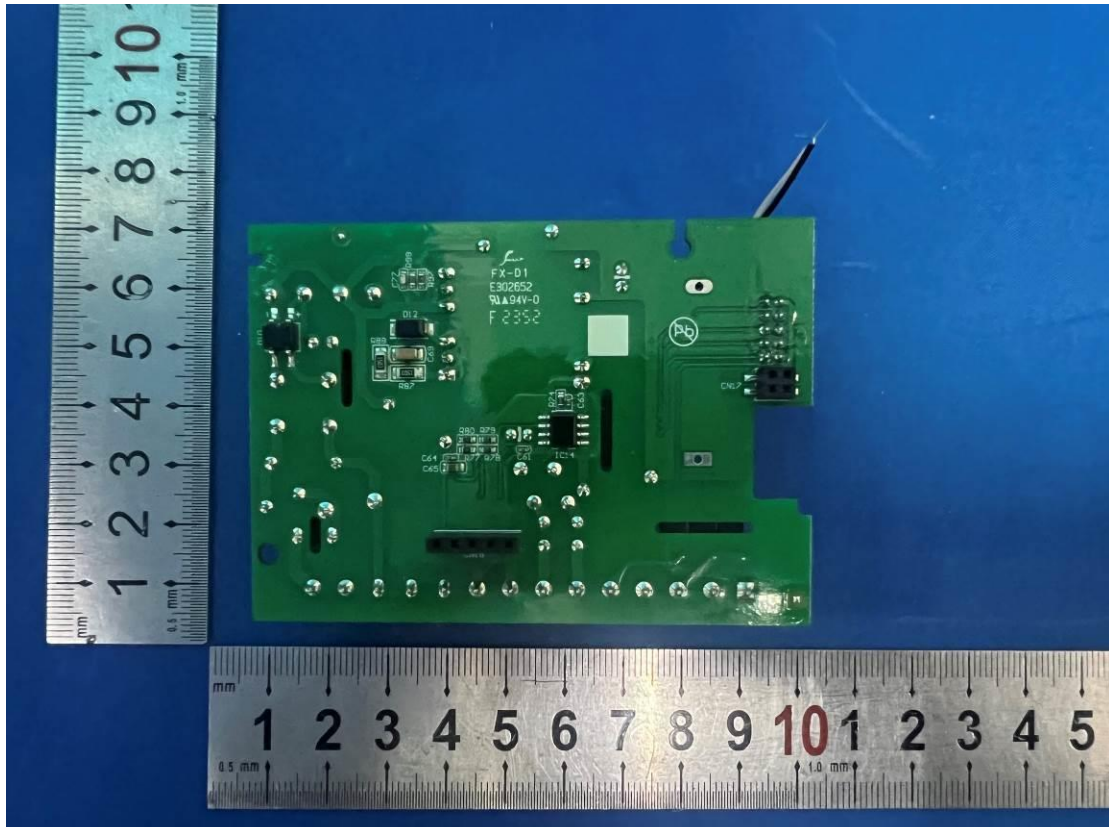
YDB072H-1 board view
