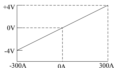
输出曲线对应图 Output Curve Diagram
