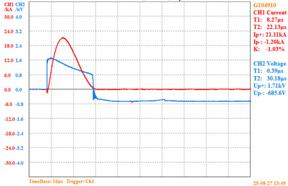
Residual voltage with 8/20 current impulses L-N mode I_n=20\text{kA} , U_p=1.8\text{kV}
